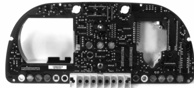
Original Battery SI Board. A battery-less replacement is not available for this model.
